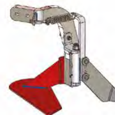
Kit lama interfilare mod. P Inter-row blade kit mod. P Kit lame ouillère mod. P Kit cuchilla intercepas mod. P
